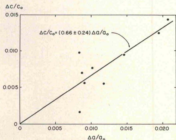
Fig. 4. Comparison between the linear compressibilities of the a axis and the c axis. The linear equation was derived by a least squares fit of all the data points.
