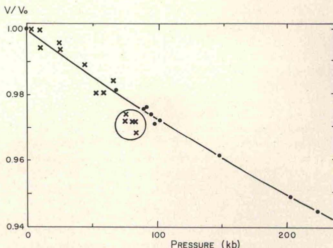
Fig. 1. The pressure dependence of the volume of stishovite at 23° ± 2°C. The solid circles are data points obtained with the diamond press for the present work; the crosses are those obtained with the tetrahedral press [Bassett and Barnett, 1970]. The circled cluster is data points believed to have been influenced by deformation of the tetrahedral press. The curve is the plot of the Birch-Murnaghan equation with K_0 = 3350 kbar and K_0' = 5.7 .
