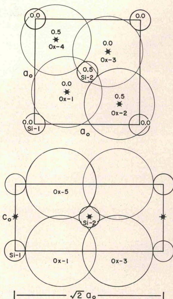
Fig. 5. The c axis projection and the (110) section of the stishovite structure. The upper number inside each atom gives the fractional distance of the atom along the axis perpendicular to the plane of the diagram. The Ox and Si represent oxygen and silicon, respectively. The radii of the circles are consistent with the ionic radii, R_{\text{Ox}} = 1.40 \text{ \AA} and R_{\text{Si}} = 0.41 \text{ \AA} [Pauling, 1960]. The value of u is 0.307 (J. S. Weaver, personal communication, 1970). The stars in the diagrams indicate the points at which chains of nearest-neighbor atoms pass through perpendicular to the planes of the diagrams.
